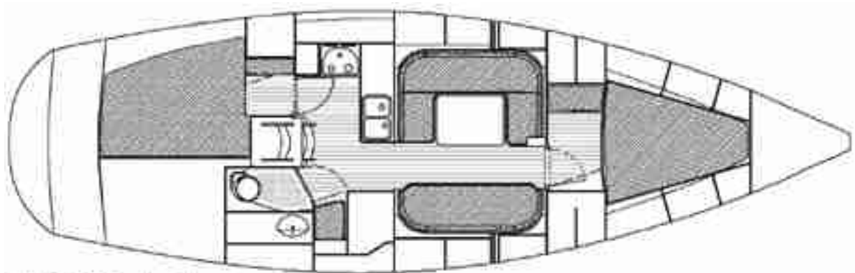
MALÖ 36 Standard layout
